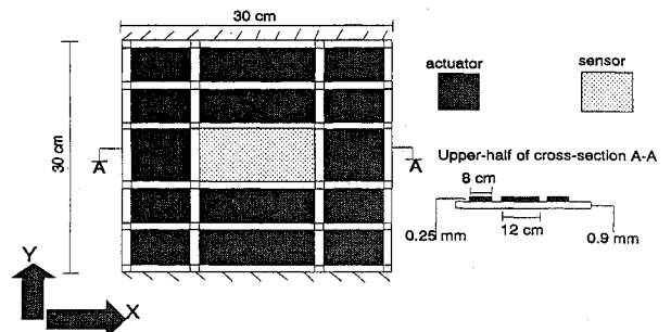
Fig. 1 Locations and sizes of PZT sensors and actuators in a "smart" plate.
